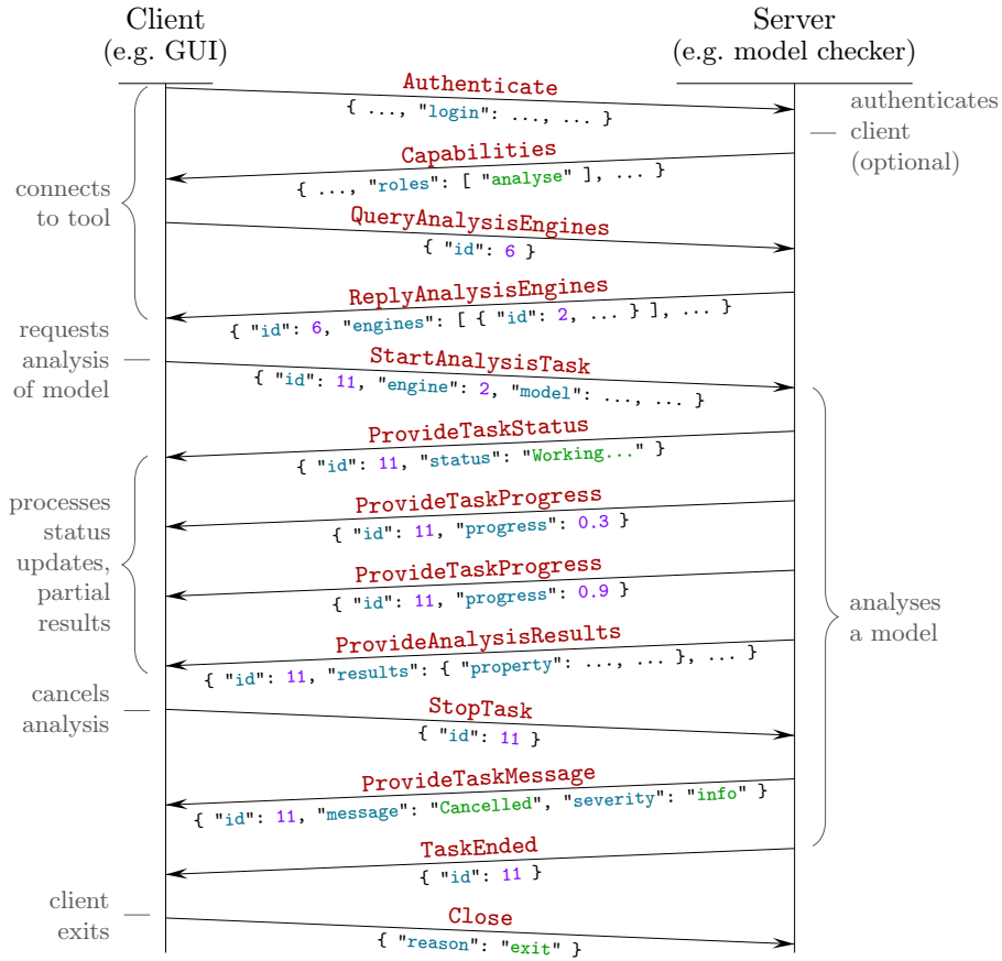
Figure 2. An example jani-interaction session
