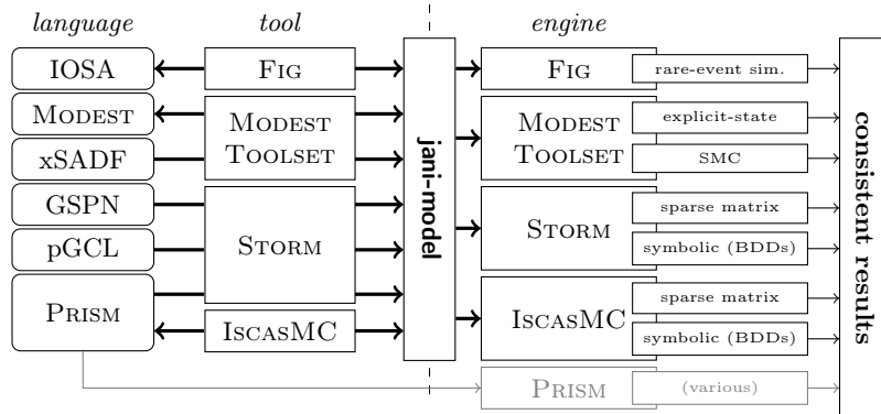
Figure 3. The JANI landscape
