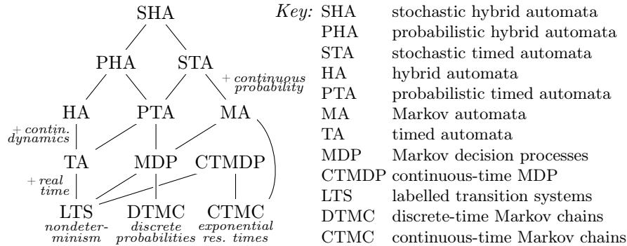
Figure 1. Model types supported by the jani-model format
